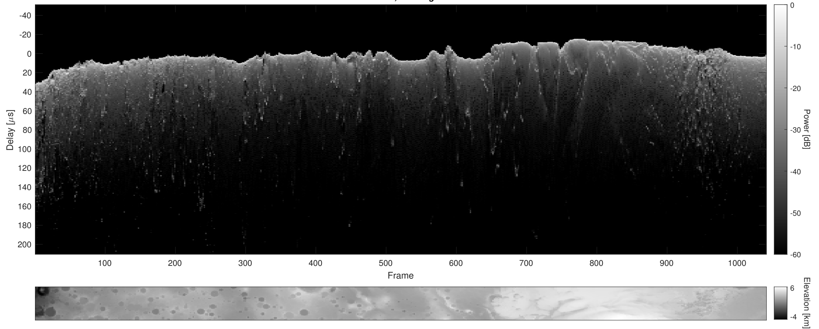
Orbit 2746, Cluttergram
