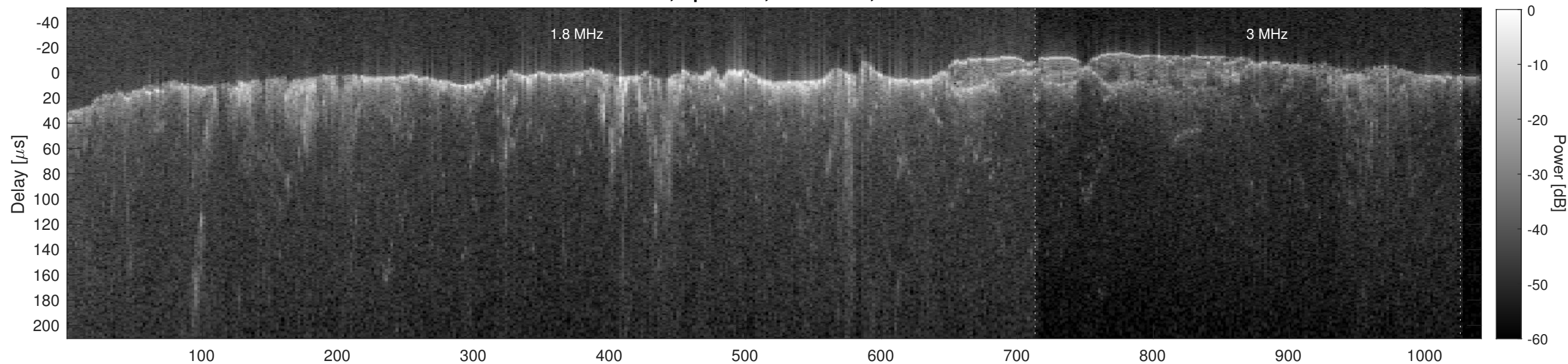
Orbit 2746, Cluttergram
