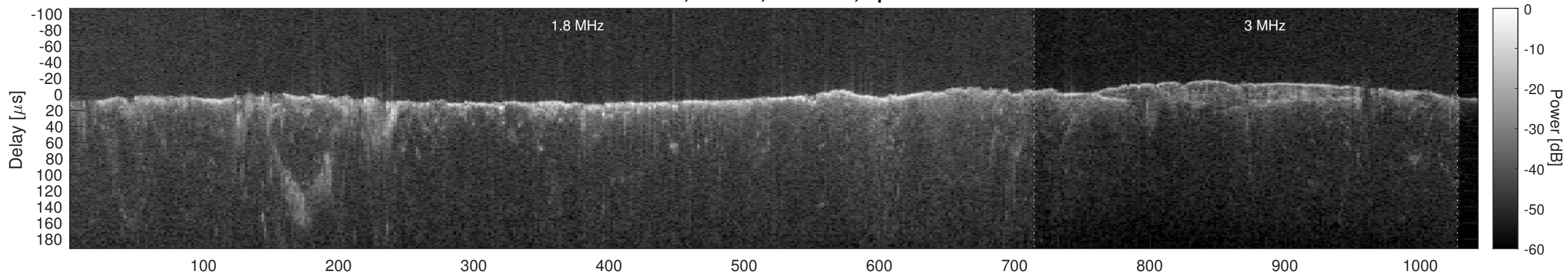
Orbit 2747, Cluttergram
