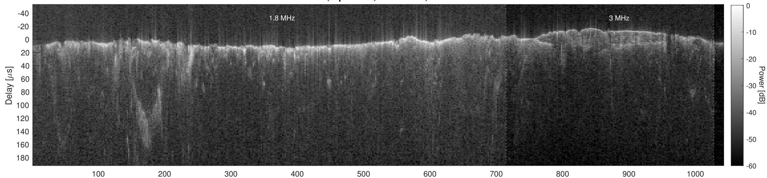
Orbit 2747, Cluttergram
