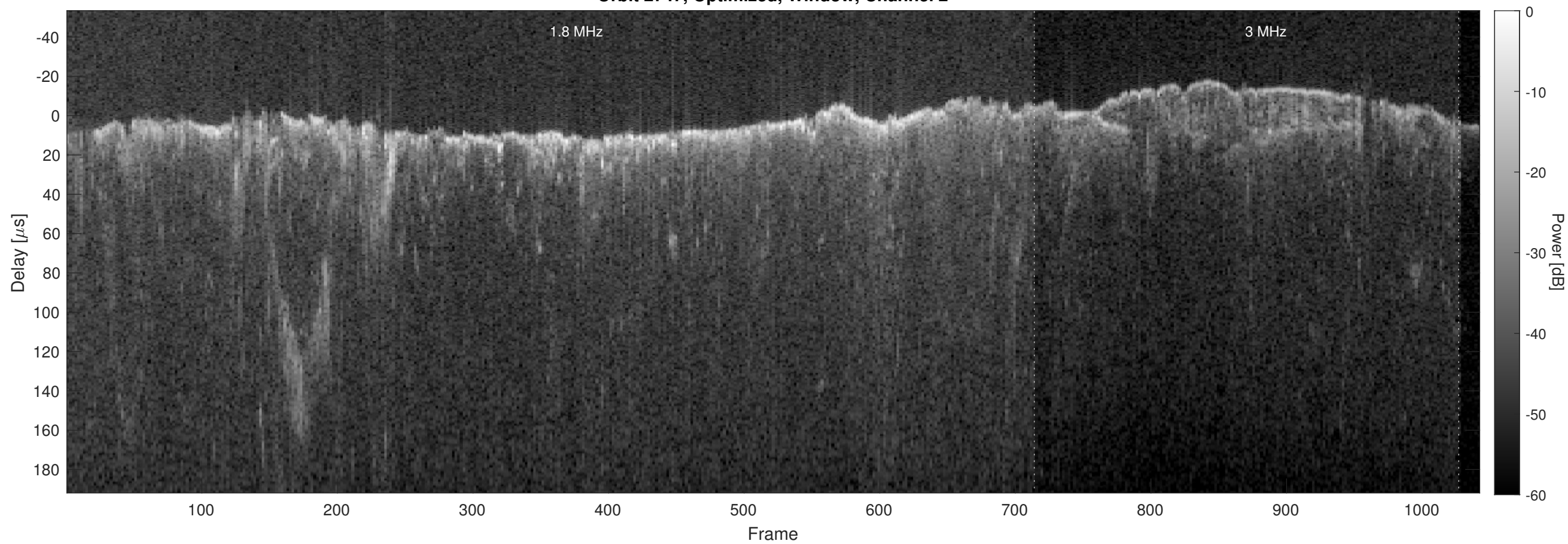
Orbit 2747, Optimized, Window, Channel 2
