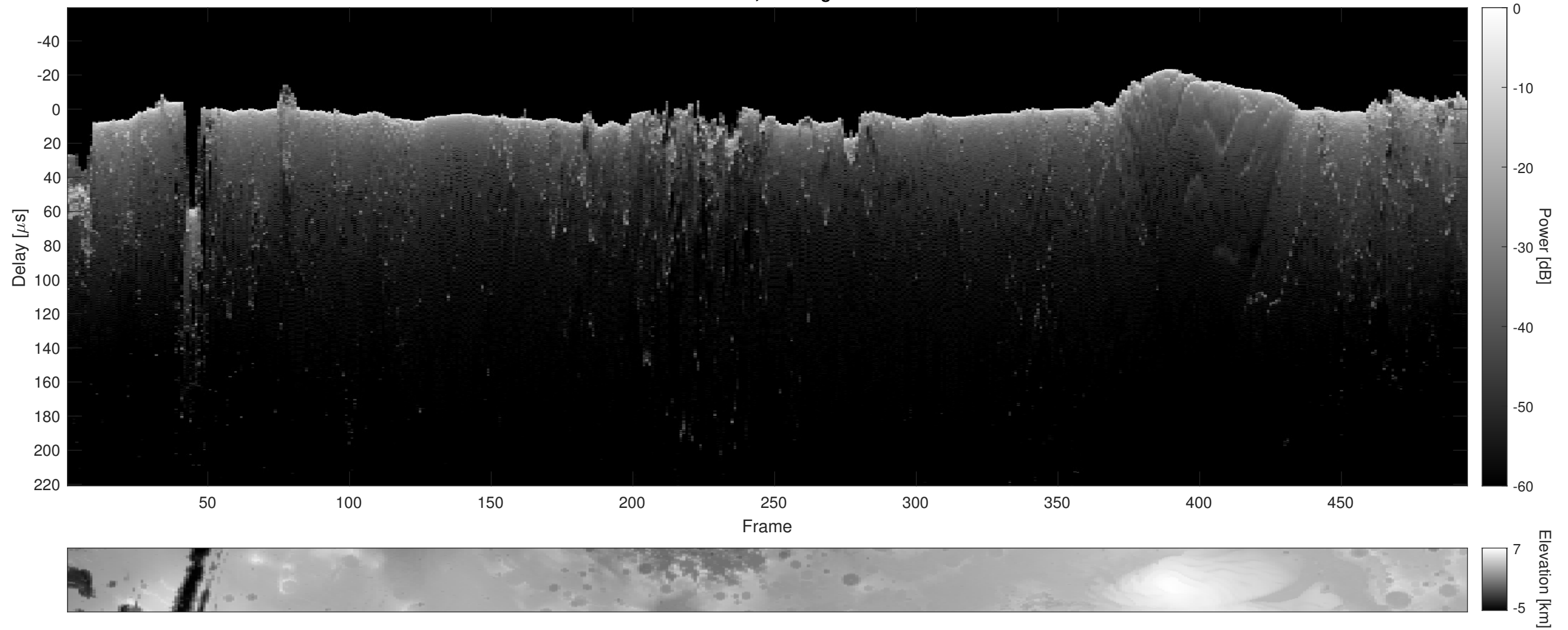
Orbit 2748, Cluttergram
