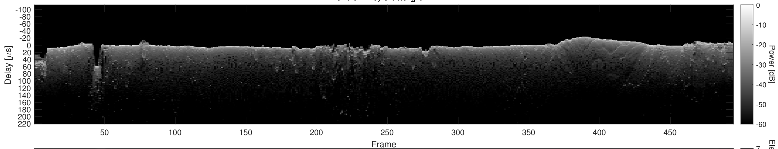
Orbit 2748, Cluttergram
