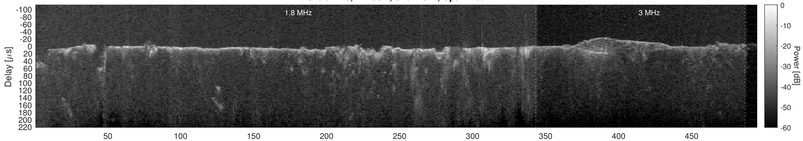
Orbit 2748, Cluttergram
