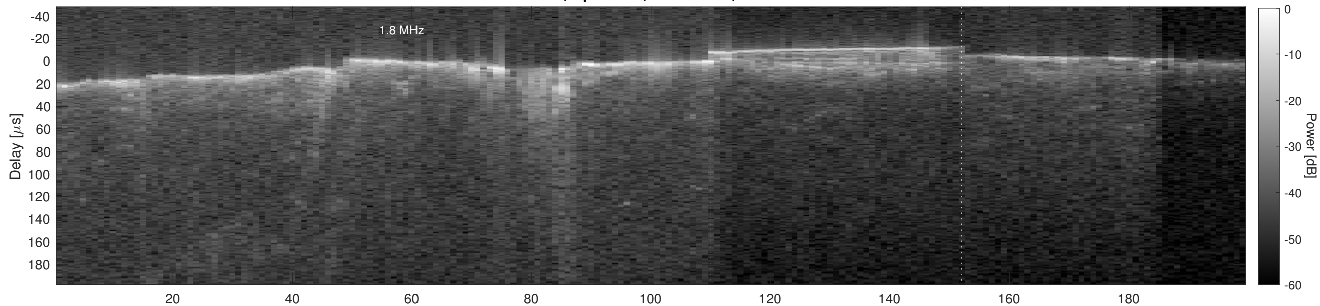
Orbit 2749, Cluttergram
