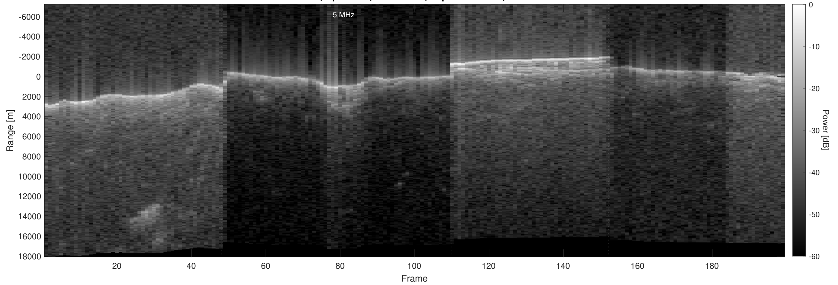
Orbit 2749, Optimized, No Window, Depth-Corrected, Channel 2
