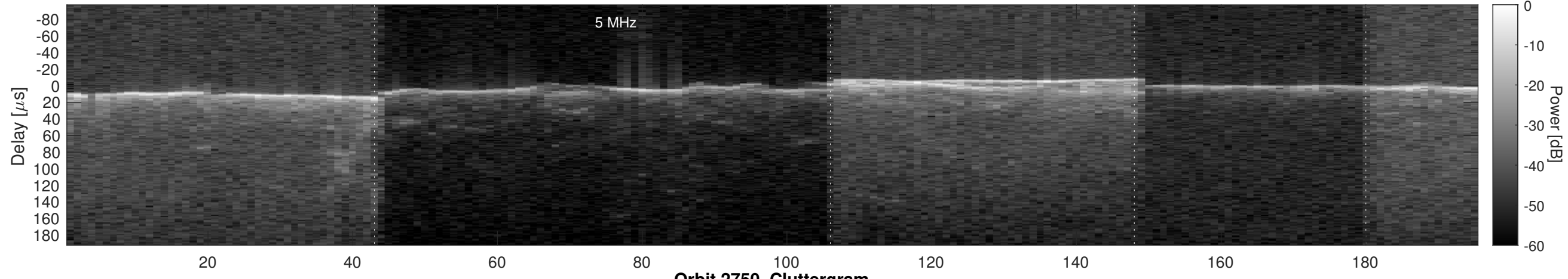
Orbit 2750, Cluttergram
