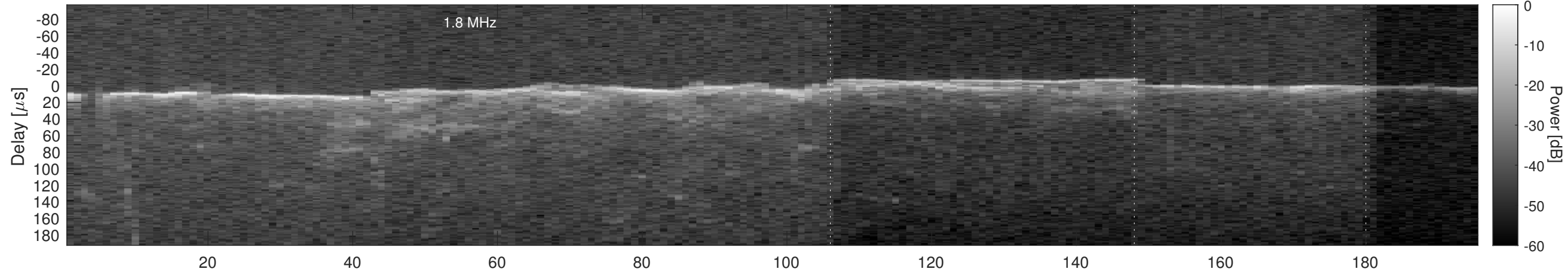
Orbit 2750, Cluttergram
