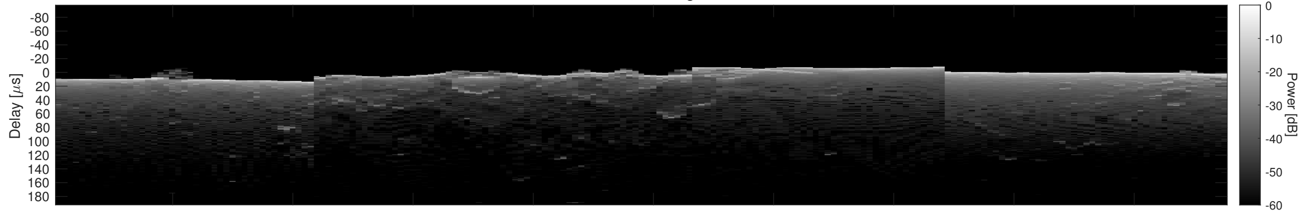
Orbit 2750, Cluttergram
