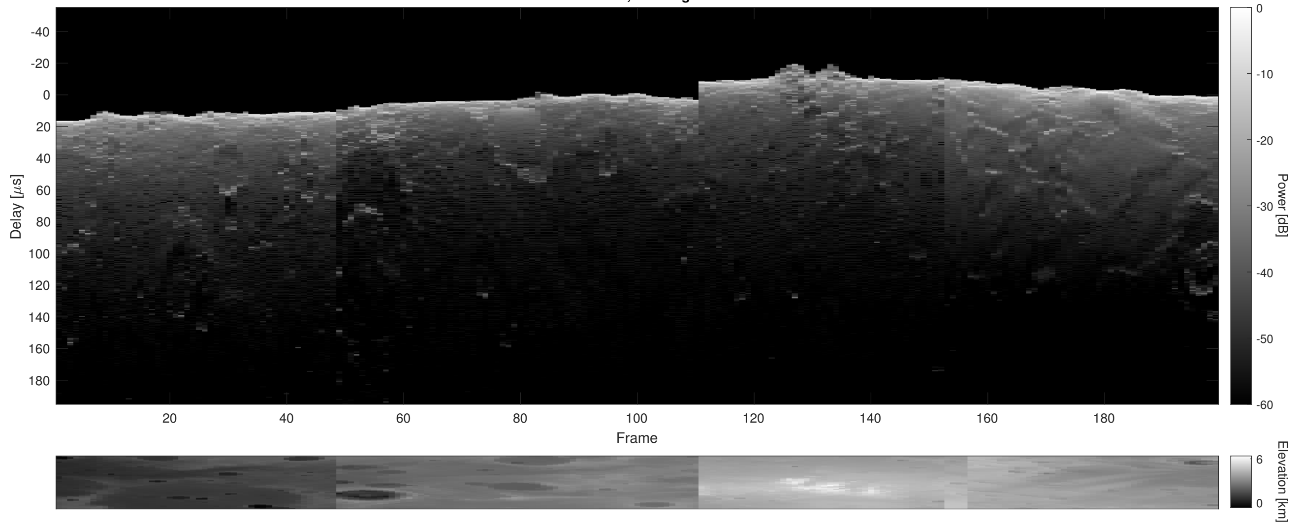
Orbit 2751, Cluttergram
