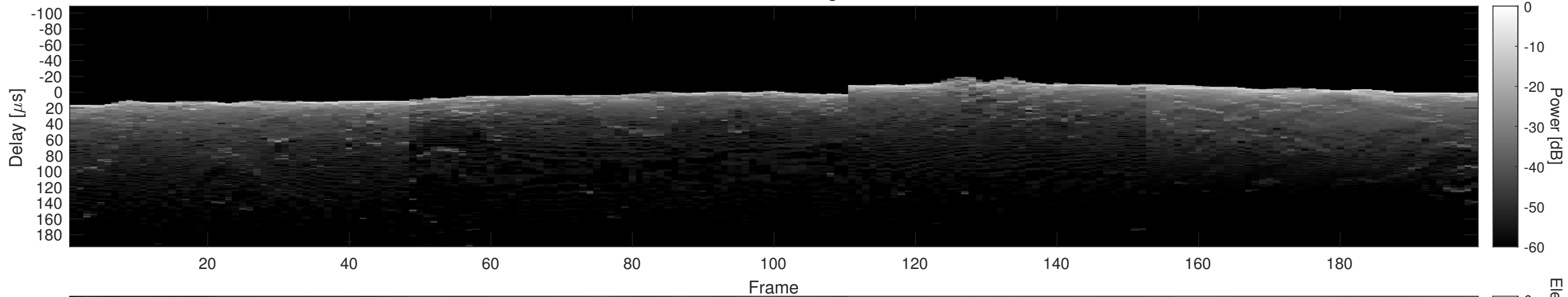
Orbit 2751, Cluttergram
