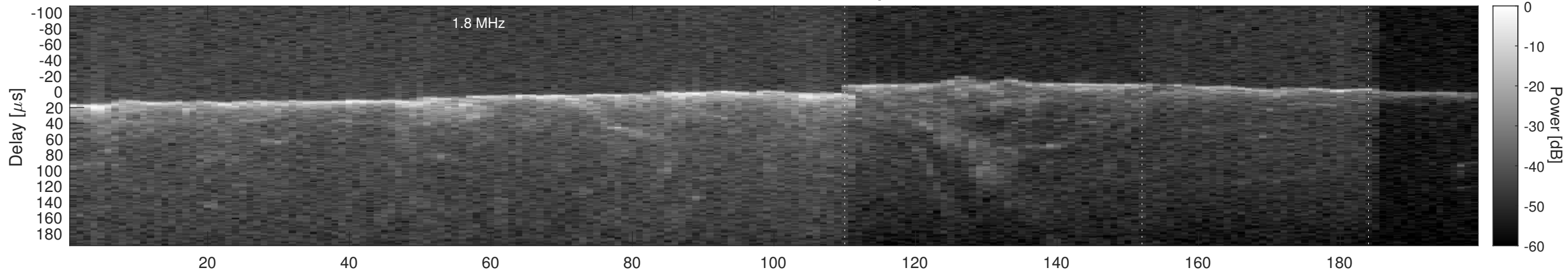
Orbit 2751, Cluttergram
