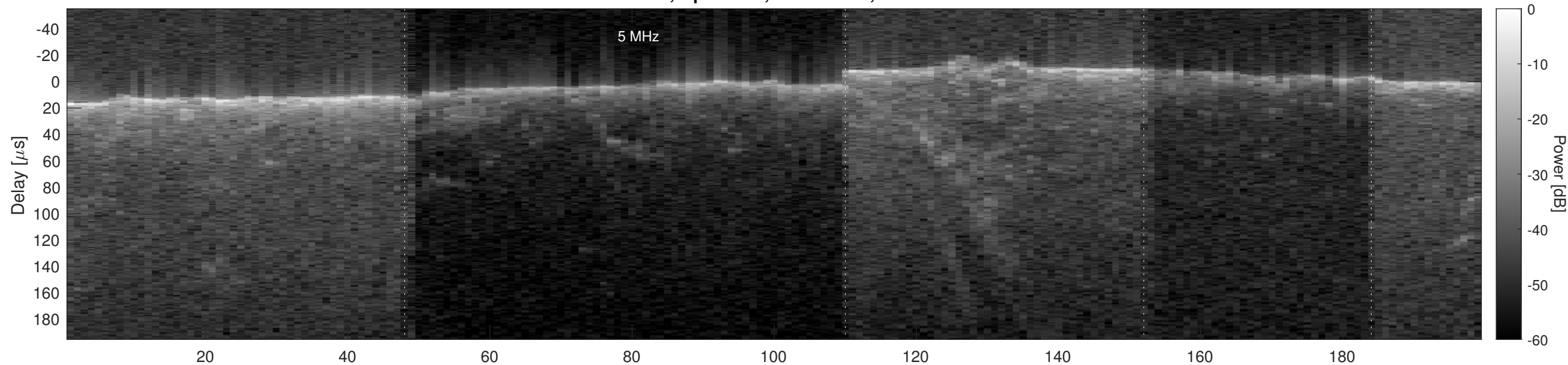
Orbit 2751, Optimized, No Window, Channel 2
