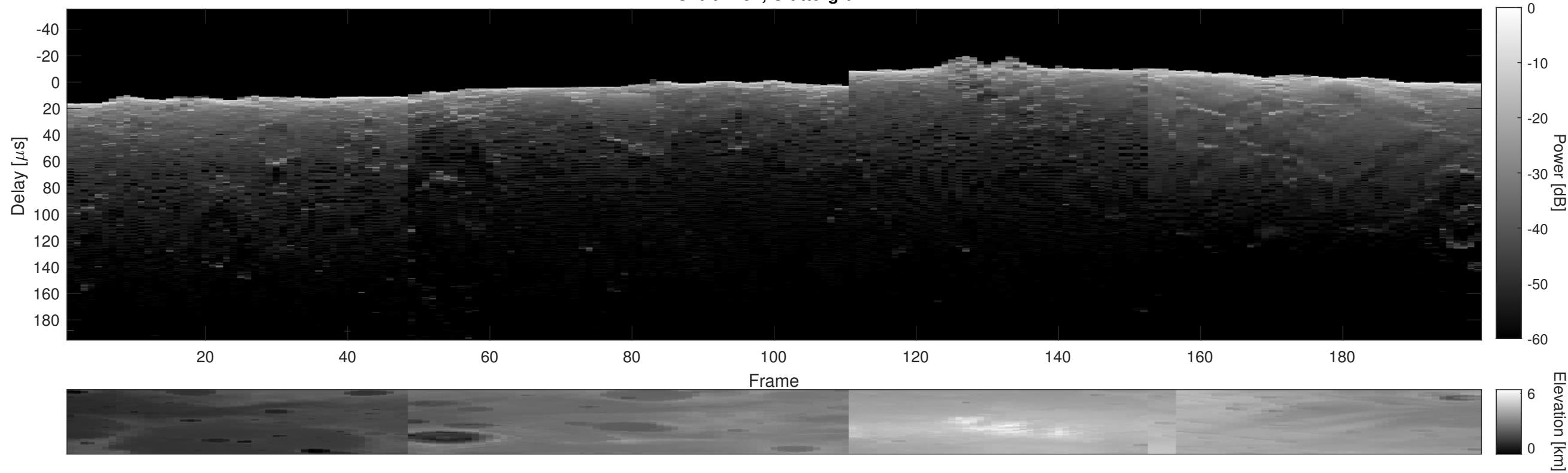
Orbit 2751, Cluttergram
