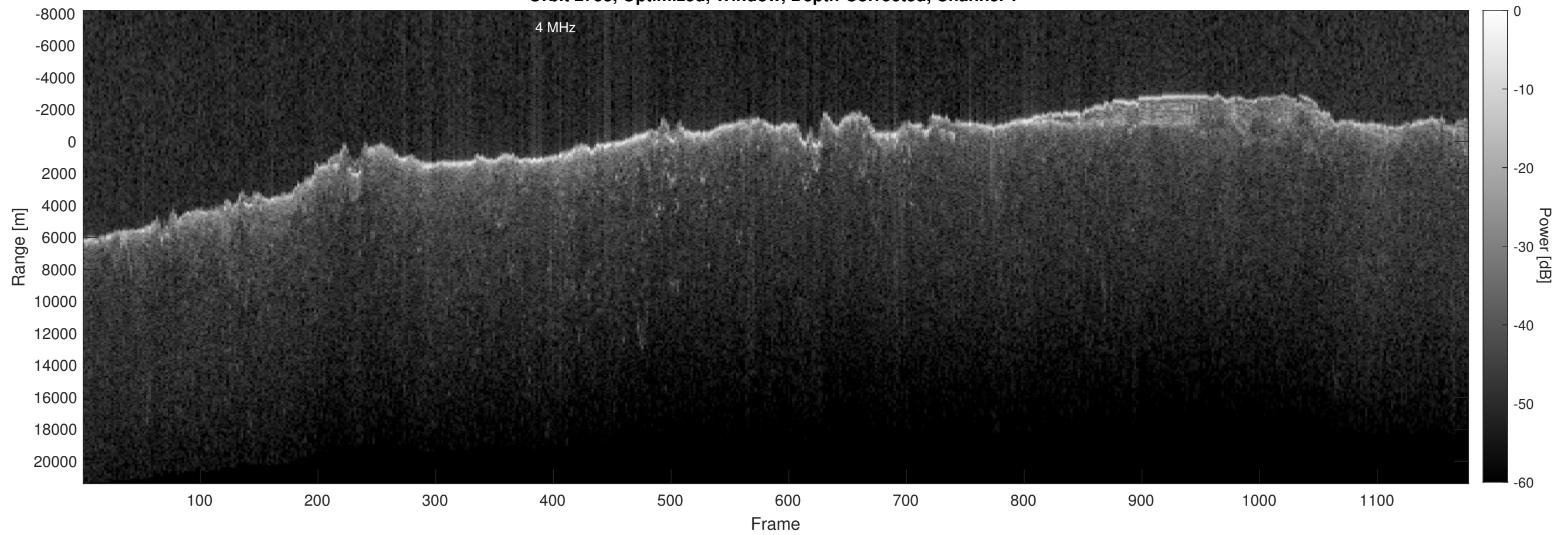
Orbit 2753, Optimized, Window, Depth-Corrected, Channel 2
