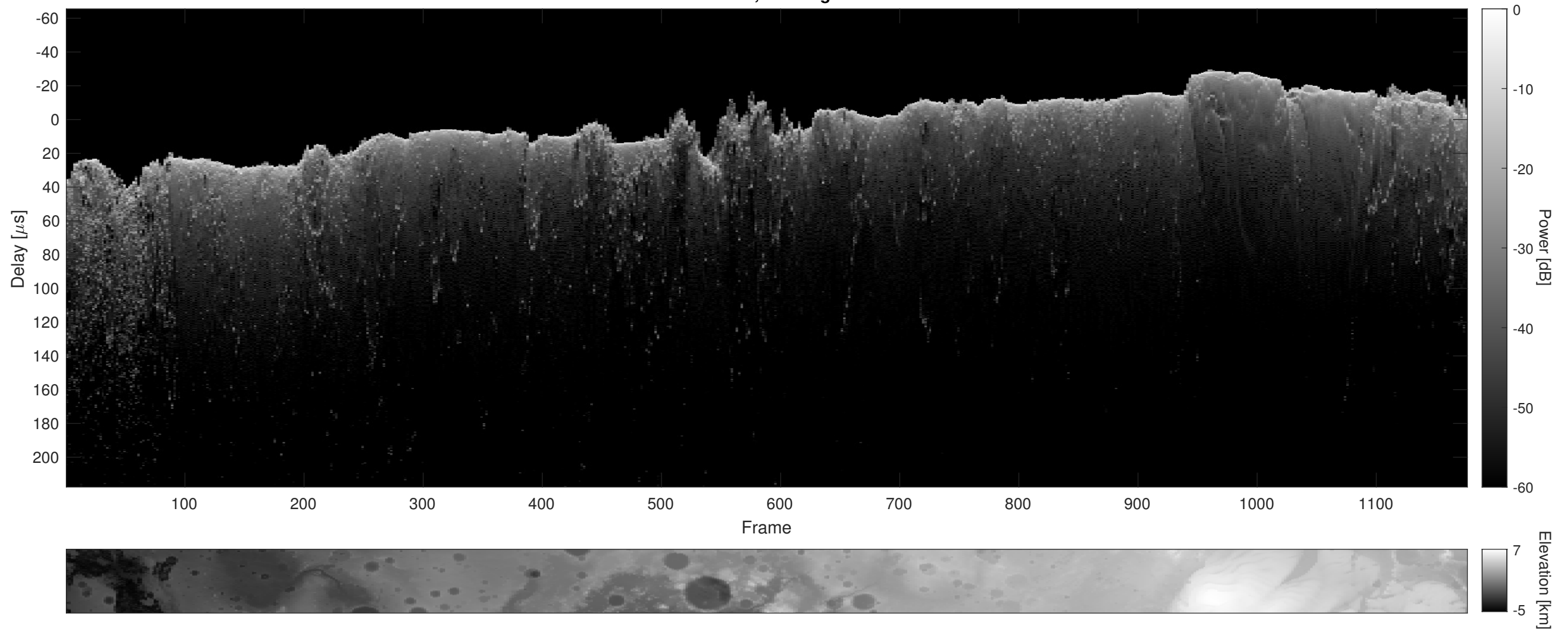
Orbit 2755, Cluttergram
