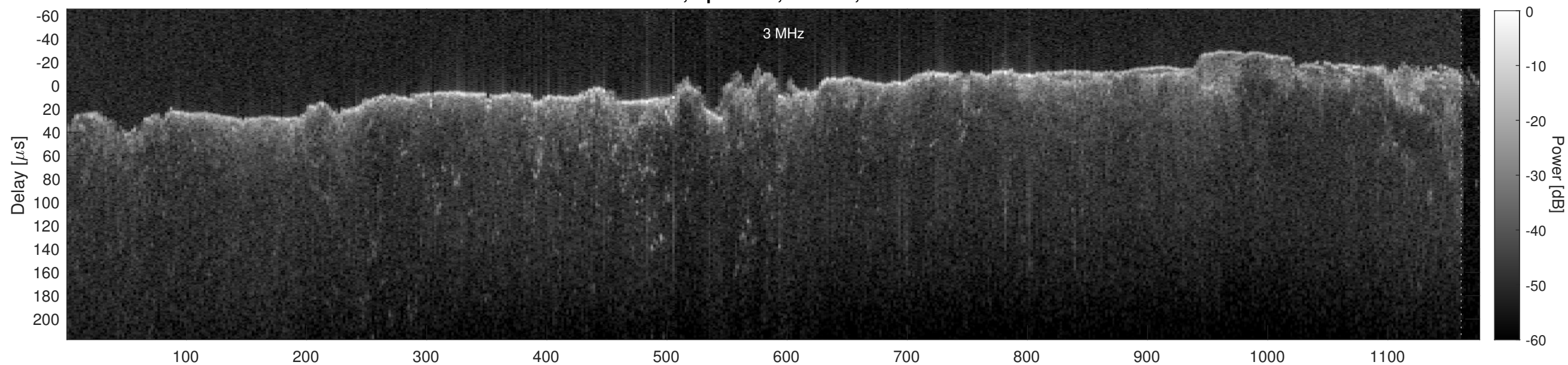
Orbit 2755, Cluttergram
