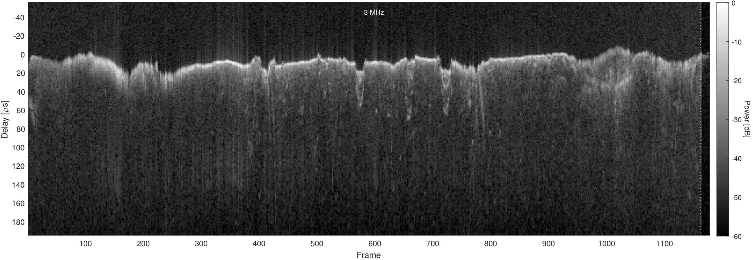
Orbit 2756, Chapman, Window, Channel 2
