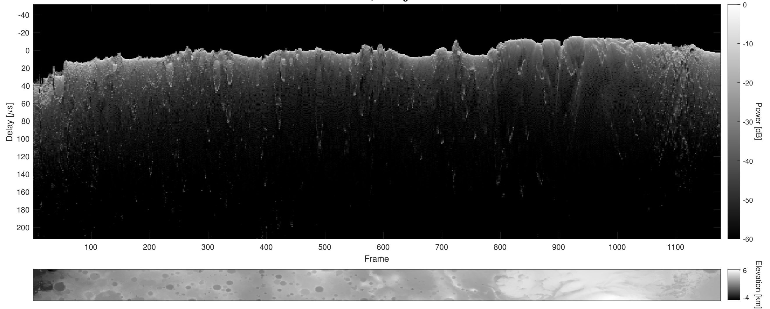
Orbit 2757, Cluttergram
