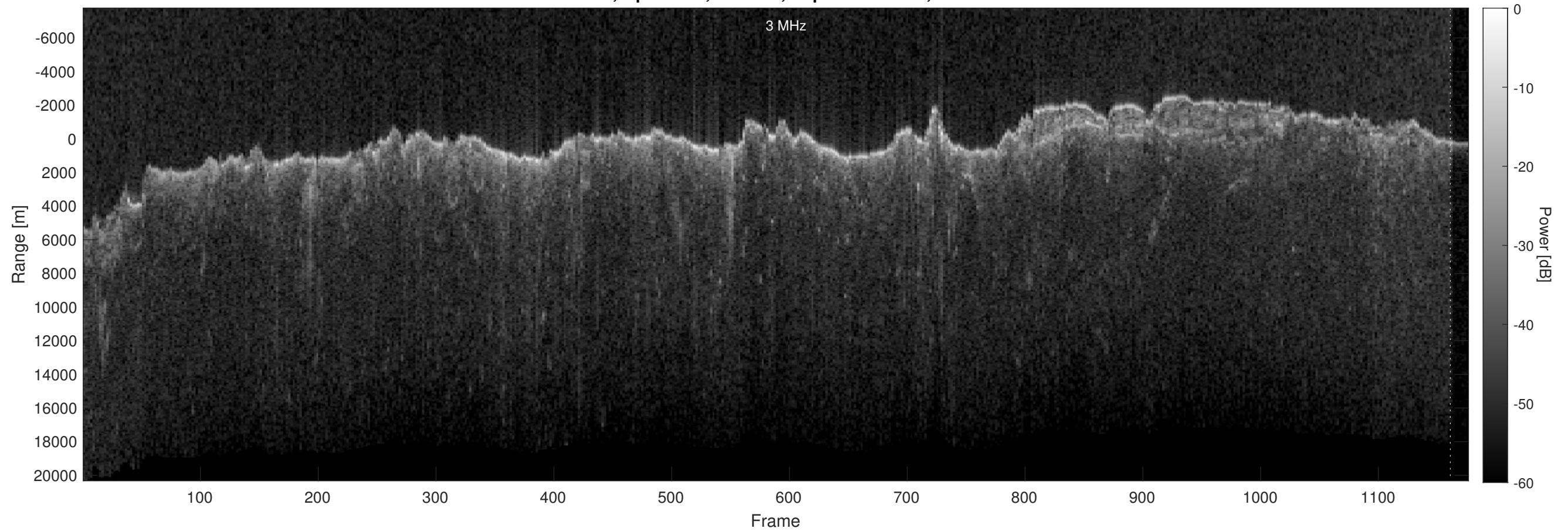
Orbit 2757, Optimized, Window, Depth-Corrected, Channel 2
