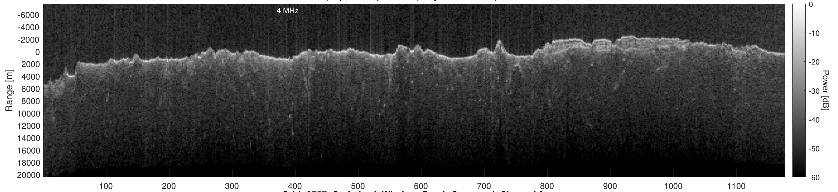
Orbit 2757, Optimized, Window, Depth-Corrected, Channel 2
