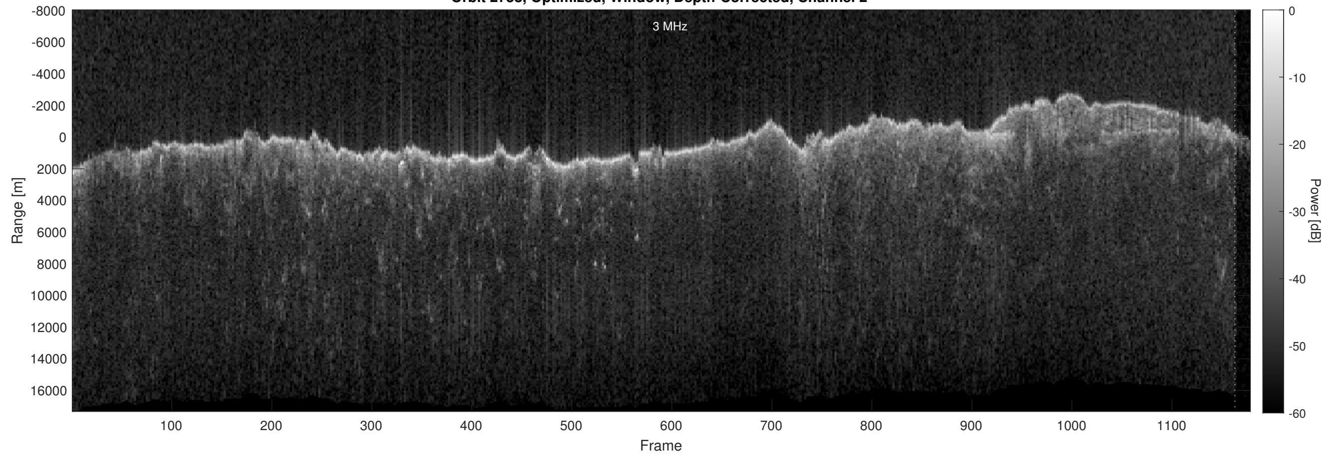
Orbit 2758, Optimized, Window, Depth-Corrected, Channel 2
