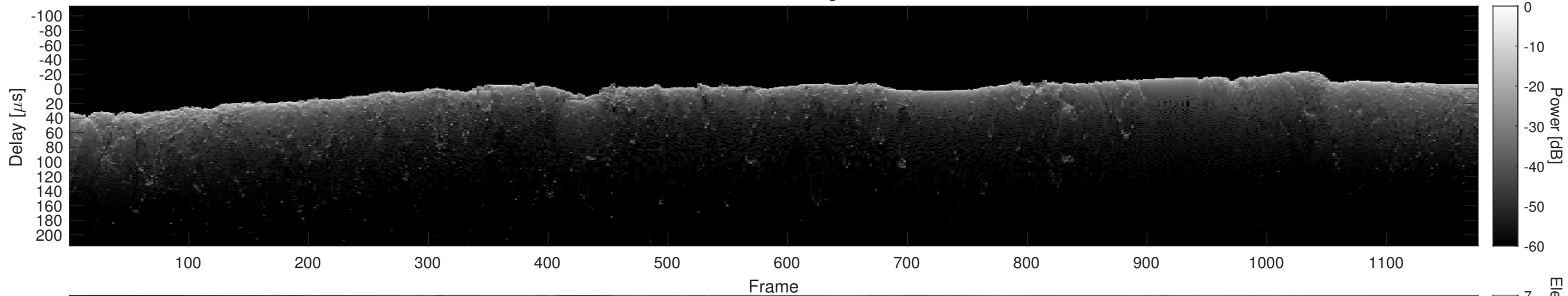
Orbit 2760, Cluttergram
