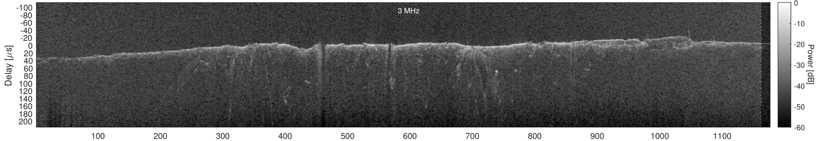
Orbit 2760, Cluttergram
