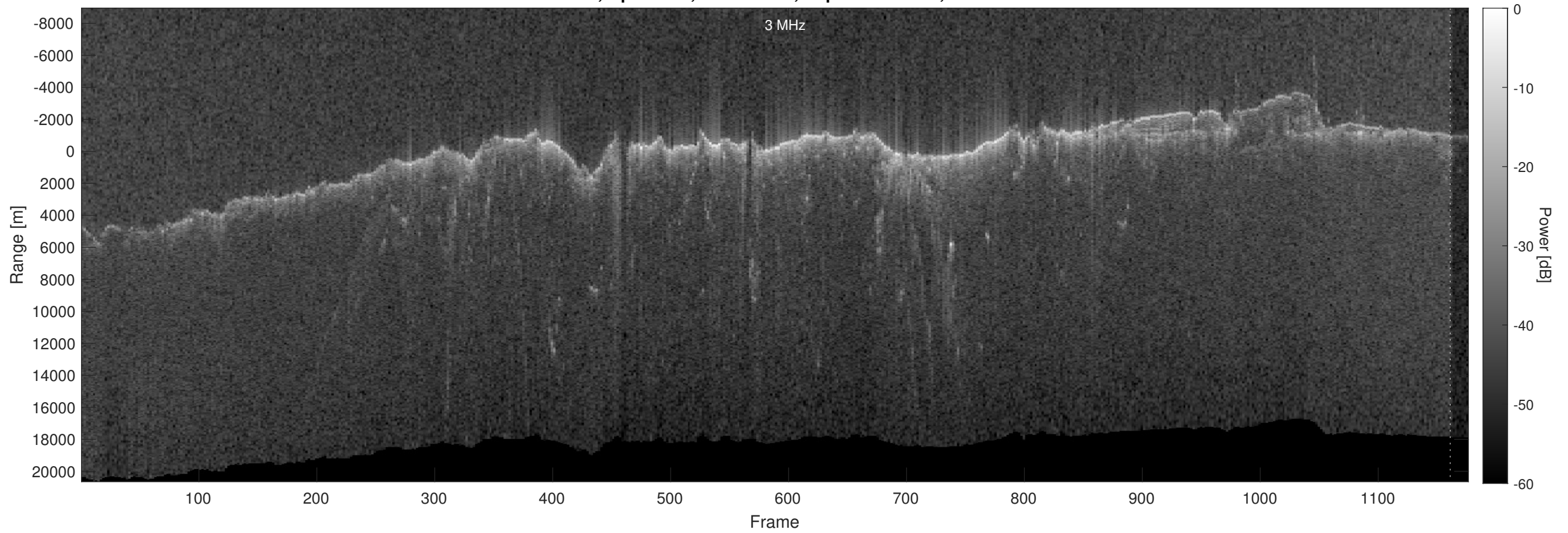
Orbit 2760, Optimized, No Window, Depth-Corrected, Channel 2
