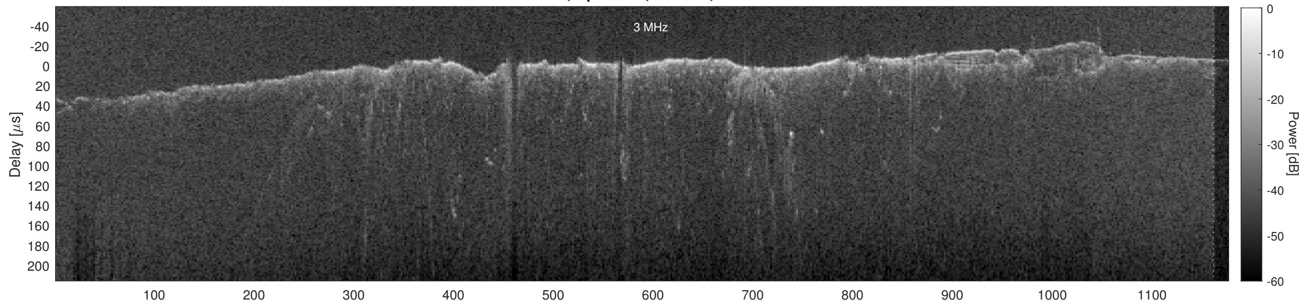
Orbit 2760, Cluttergram
