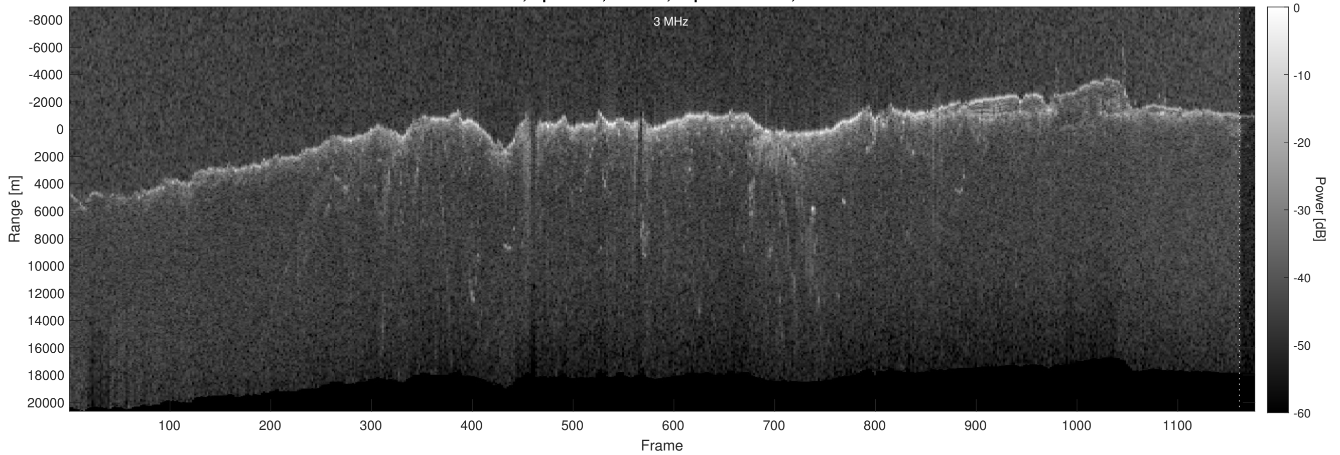
Orbit 2760, Optimized, Window, Depth-Corrected, Channel 2
