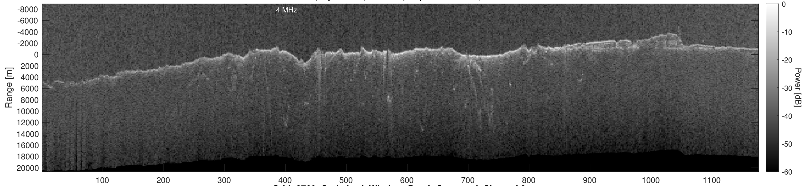
Orbit 2760, Optimized, Window, Depth-Corrected, Channel 2
