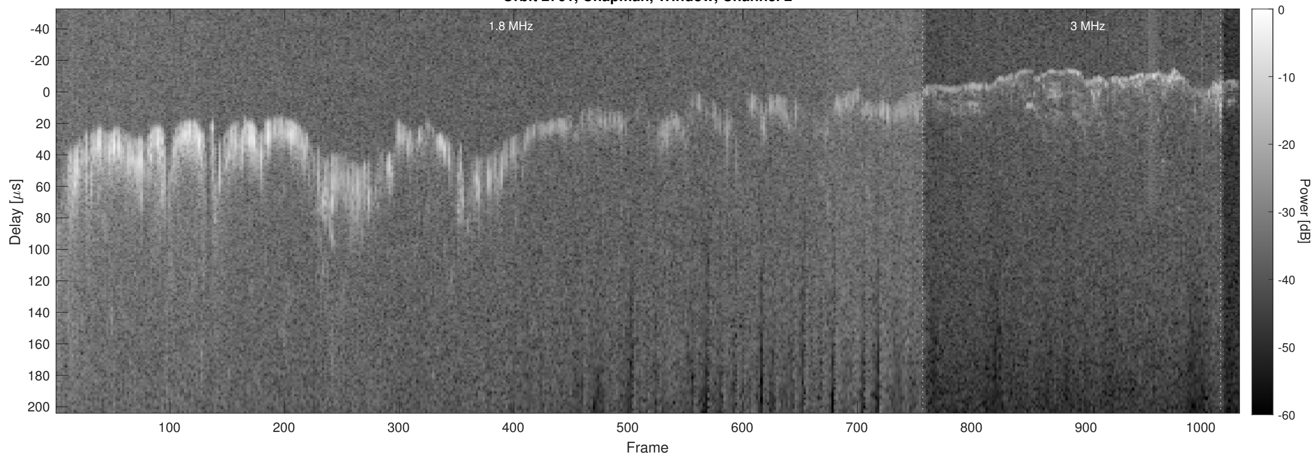
Orbit 2761, Chapman, Window, Channel 2
