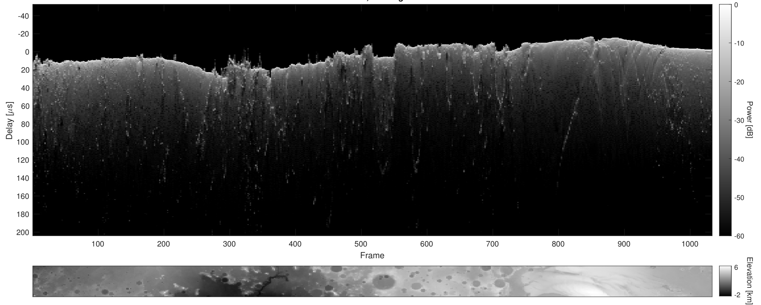
Orbit 2761, Cluttergram
