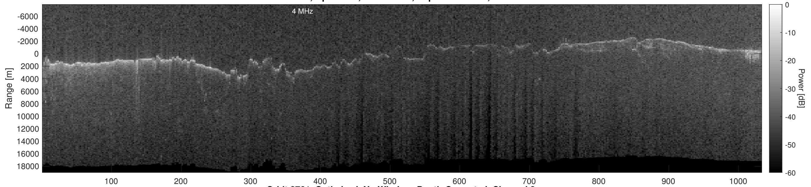
Orbit 2761, Optimized, No Window, Depth-Corrected, Channel 2
