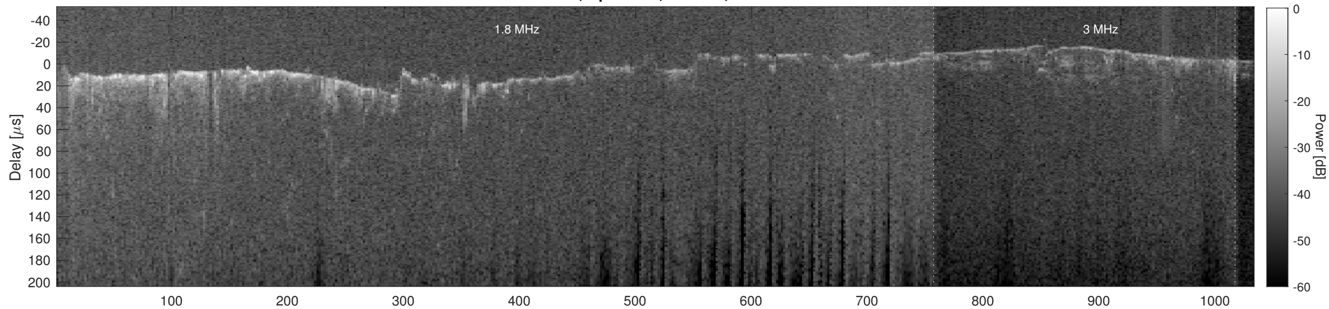
Orbit 2761, Cluttergram
