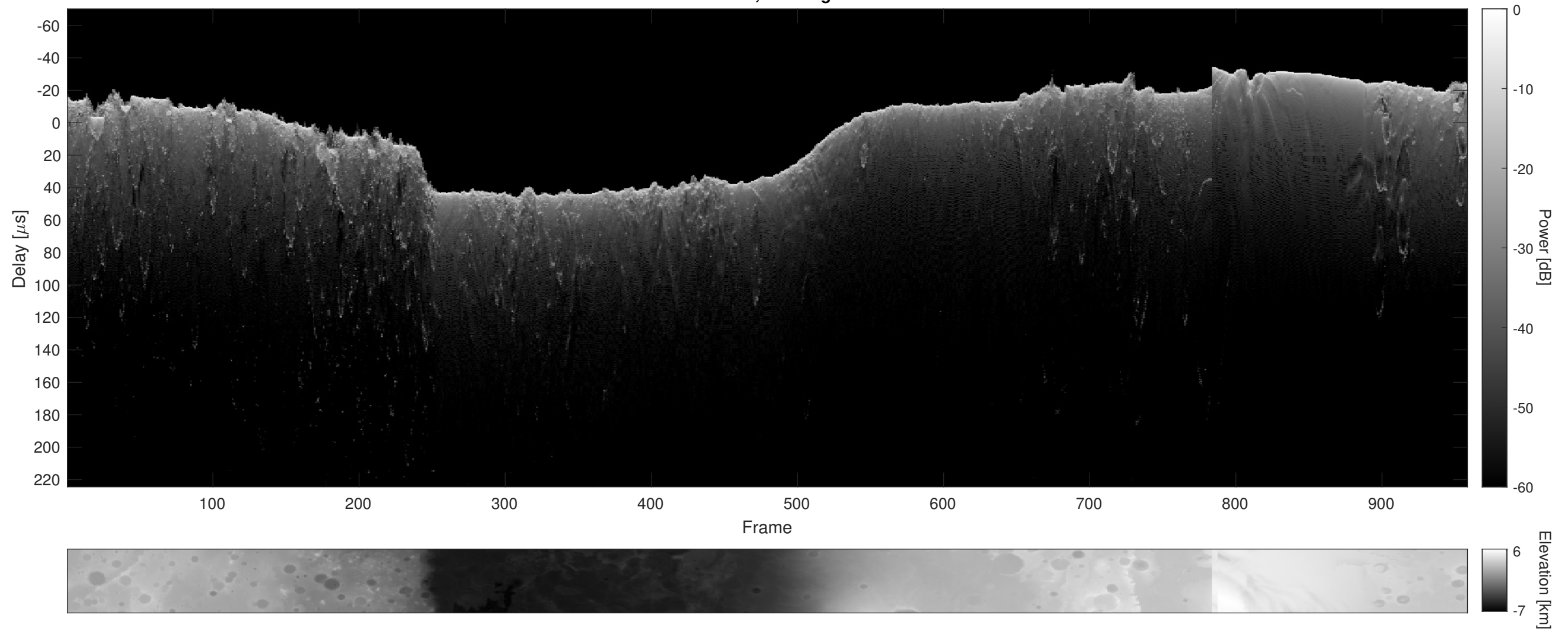
Orbit 2765, Cluttergram
