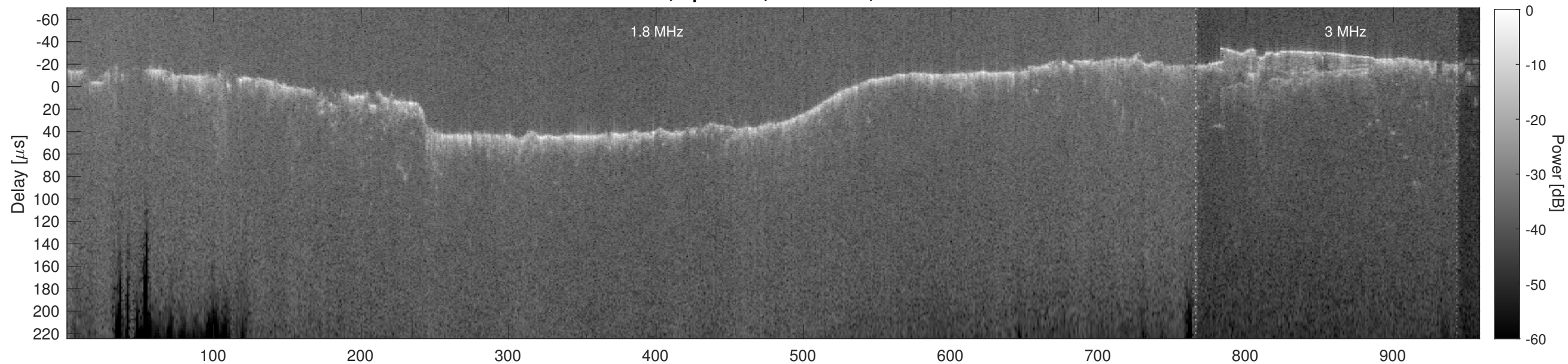
Orbit 2765, Cluttergram
