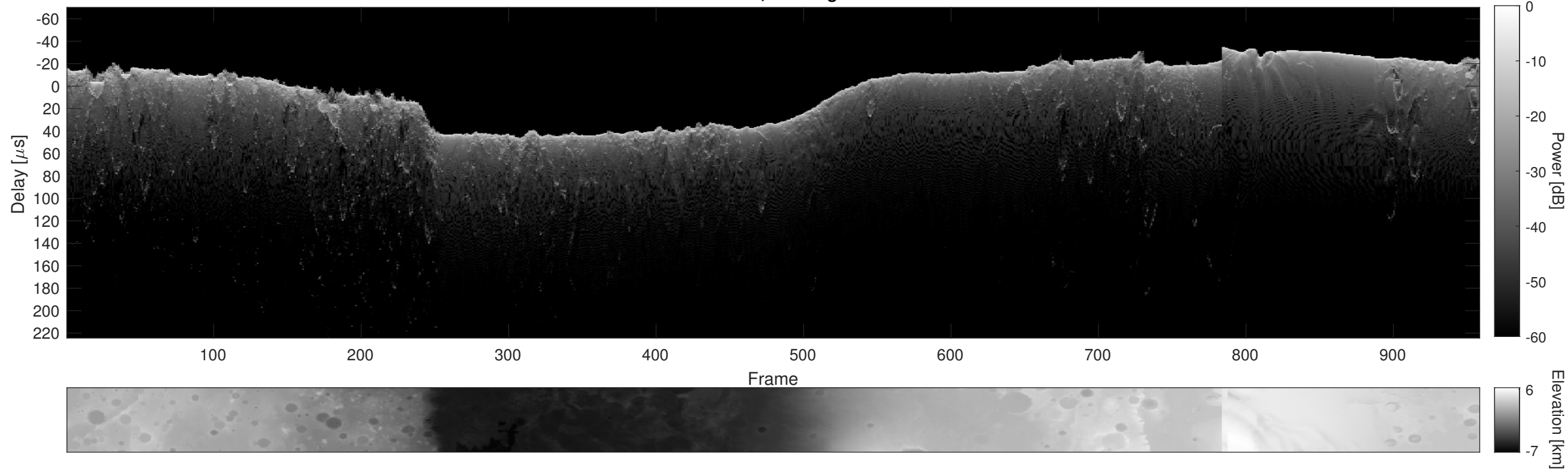
Orbit 2765, Cluttergram
