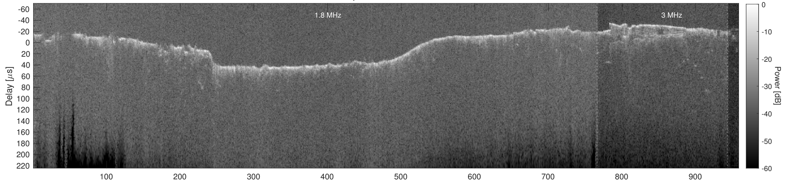
Orbit 2765, Cluttergram
