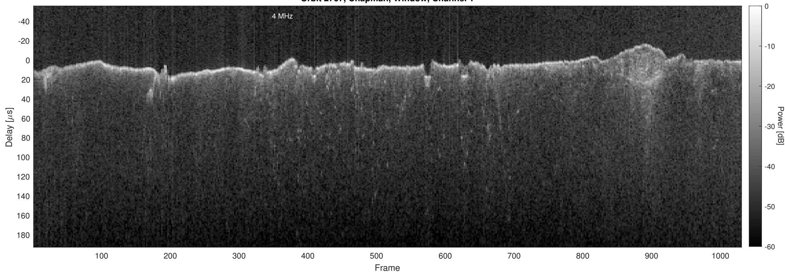
Orbit 2767, Chapman, Window, Channel 2
