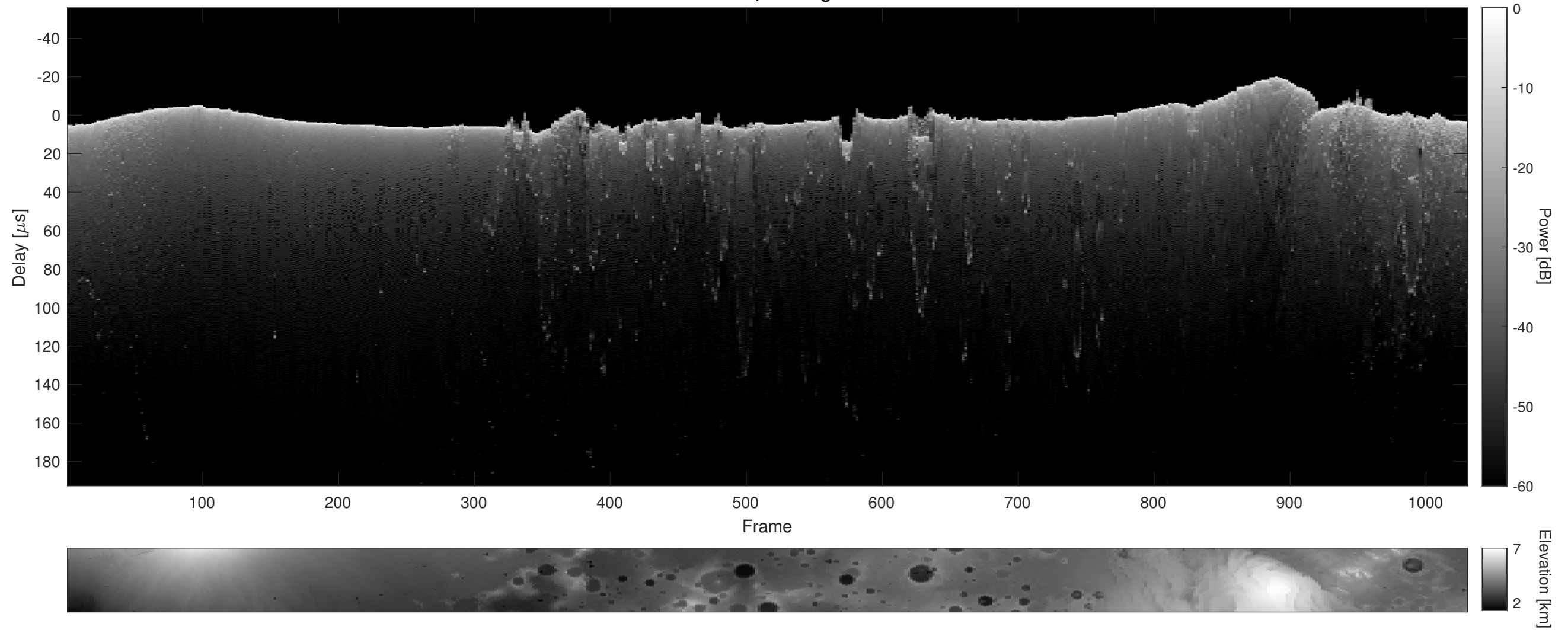
Orbit 2767, Cluttergram
