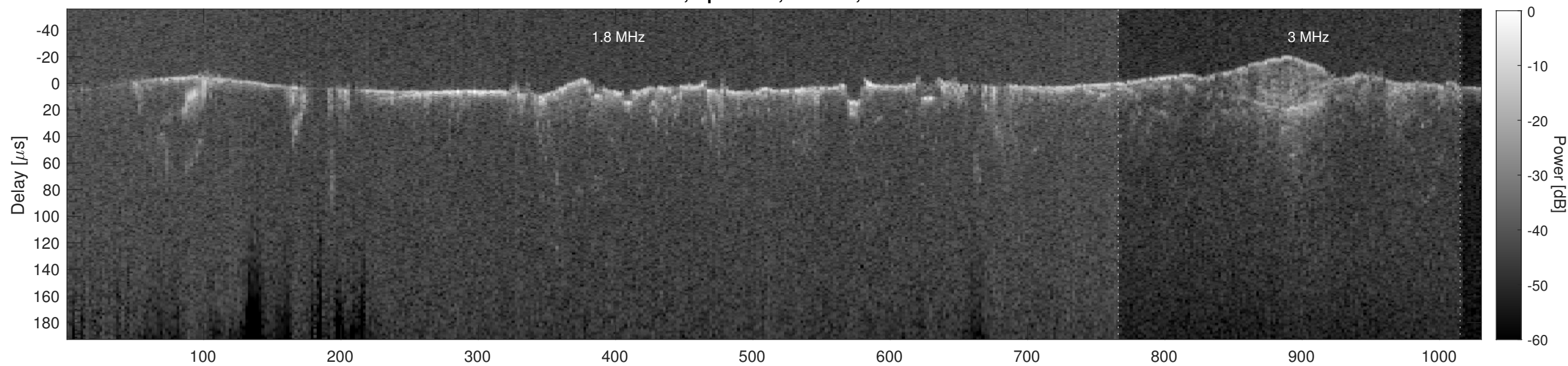
Orbit 2767, Cluttergram
