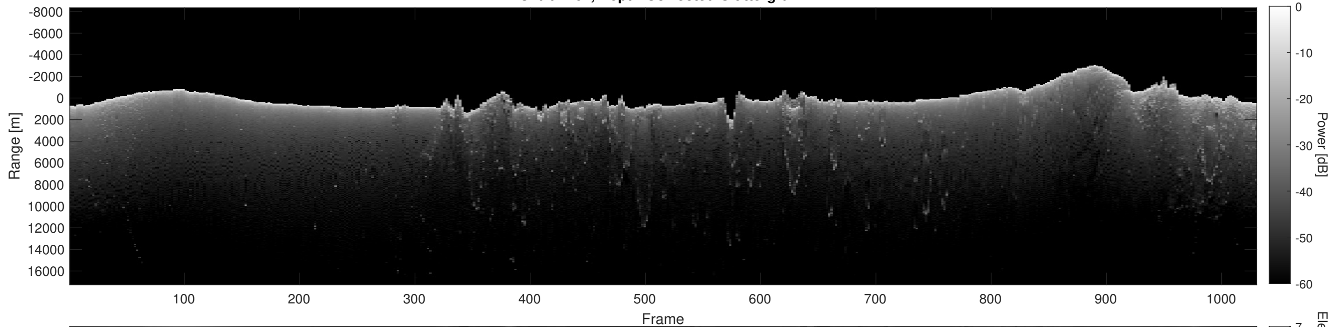
Orbit 2767, Depth-Corrected Cluttergram
