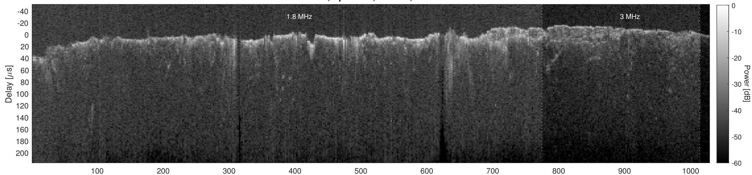
Orbit 2768, Cluttergram
