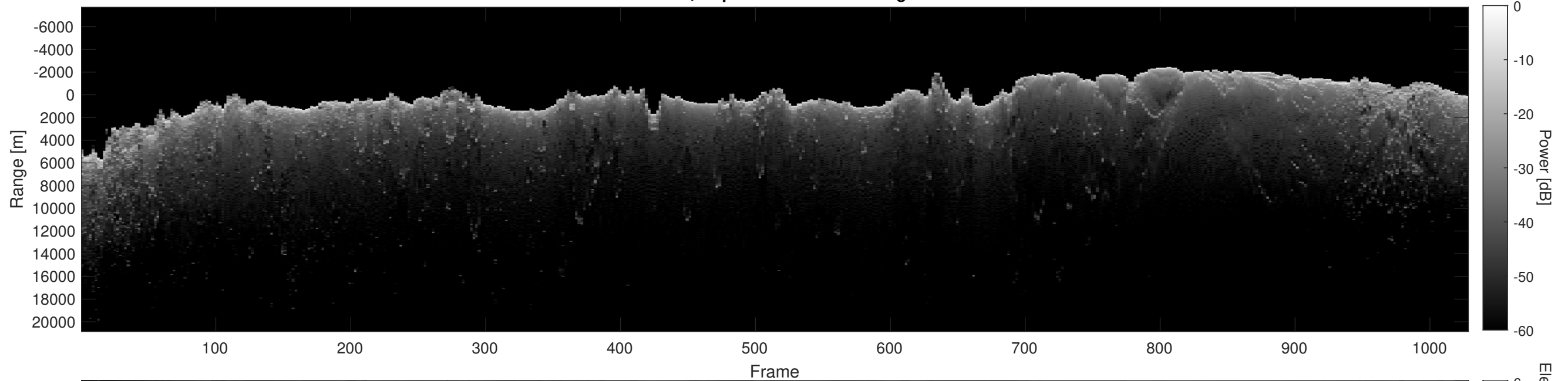
Orbit 2768, Depth-Corrected Cluttergram
