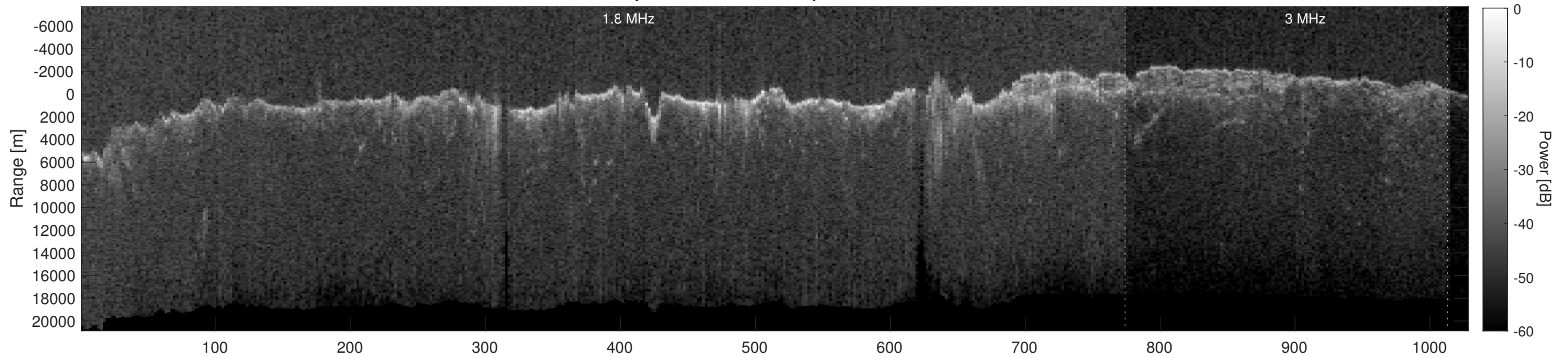
Orbit 2768, Depth-Corrected Cluttergram
