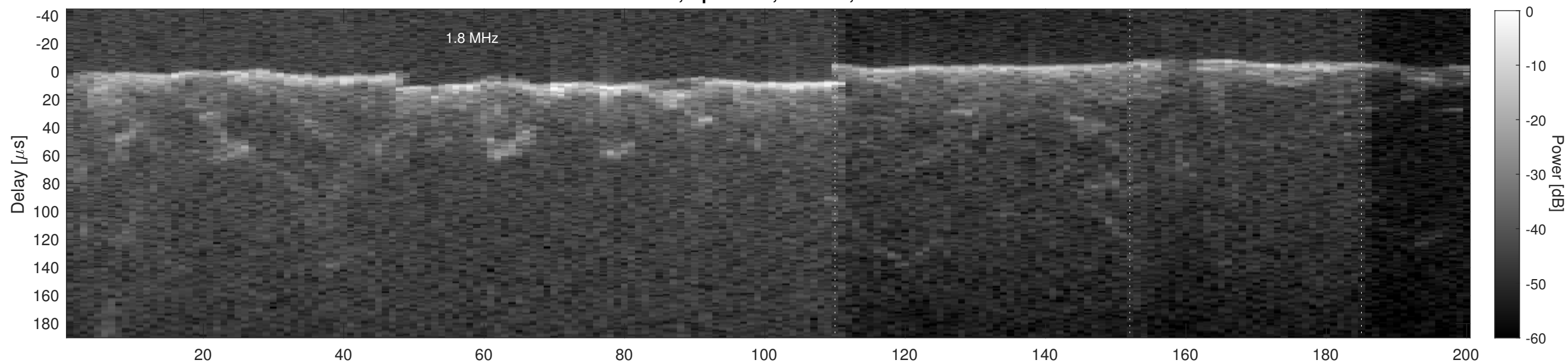
Orbit 2769, Cluttergram
