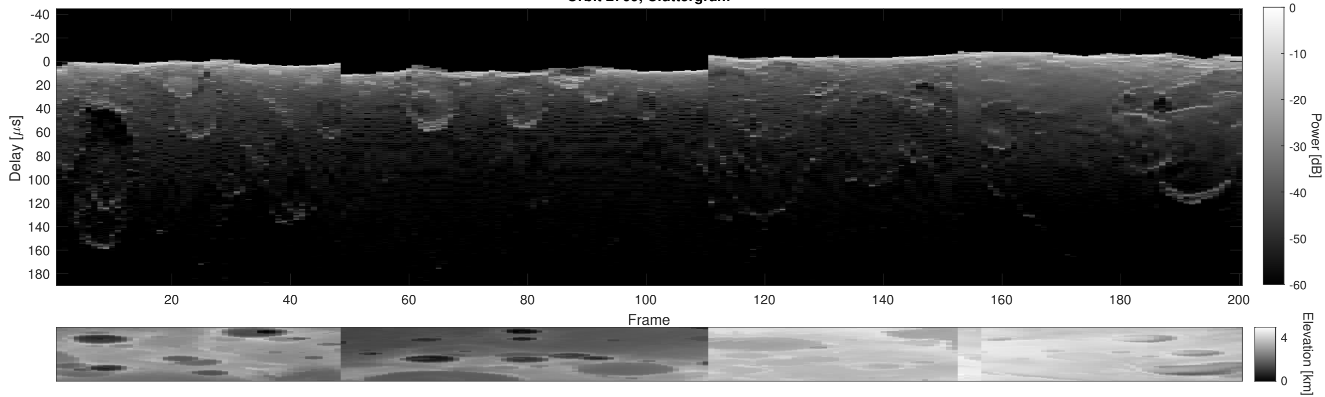
Orbit 2769, Cluttergram
