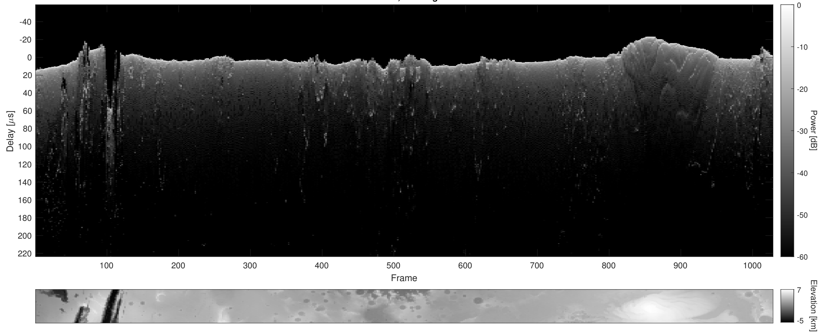
Orbit 2770, Cluttergram
