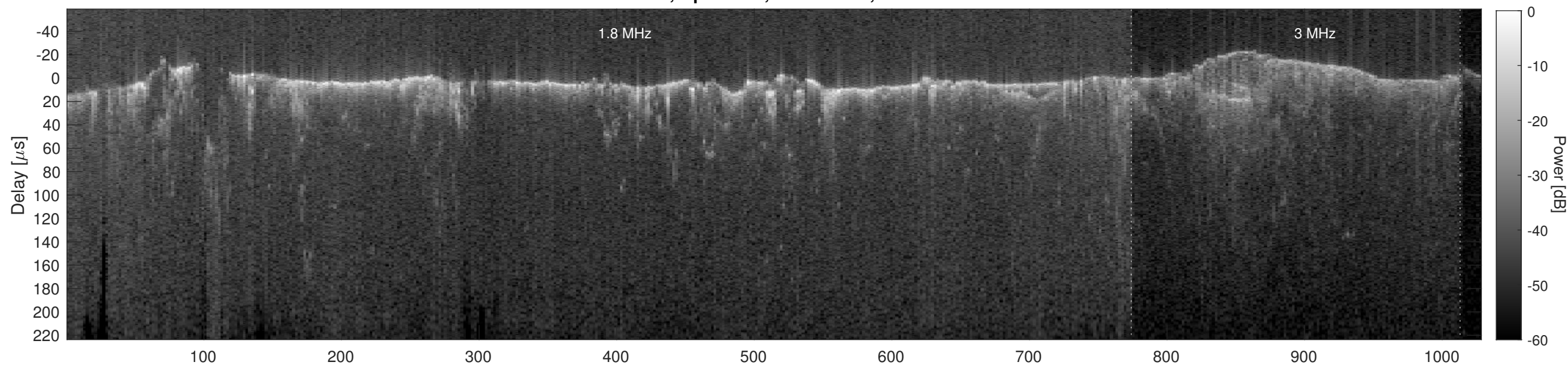
Orbit 2770, Cluttergram
