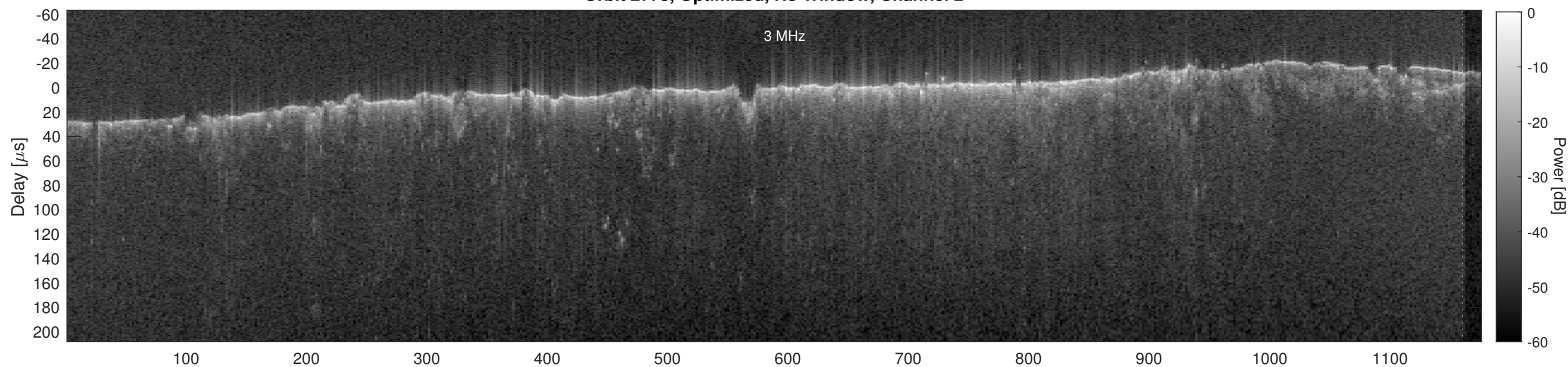
Orbit 2773, Cluttergram
