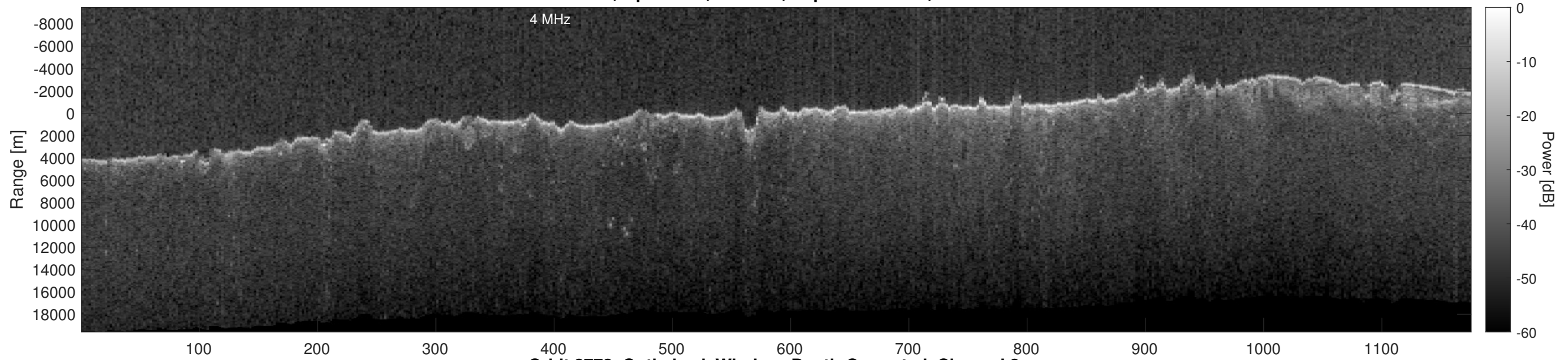
Orbit 2773, Optimized, Window, Depth-Corrected, Channel 2
