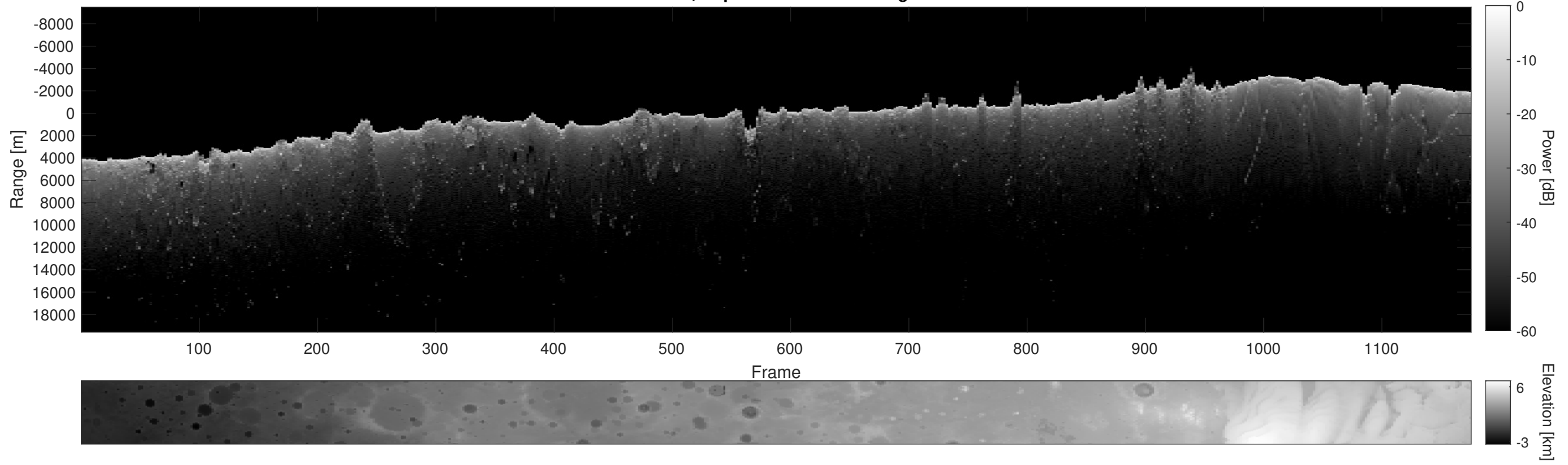
Orbit 2773, Depth-Corrected Cluttergram
