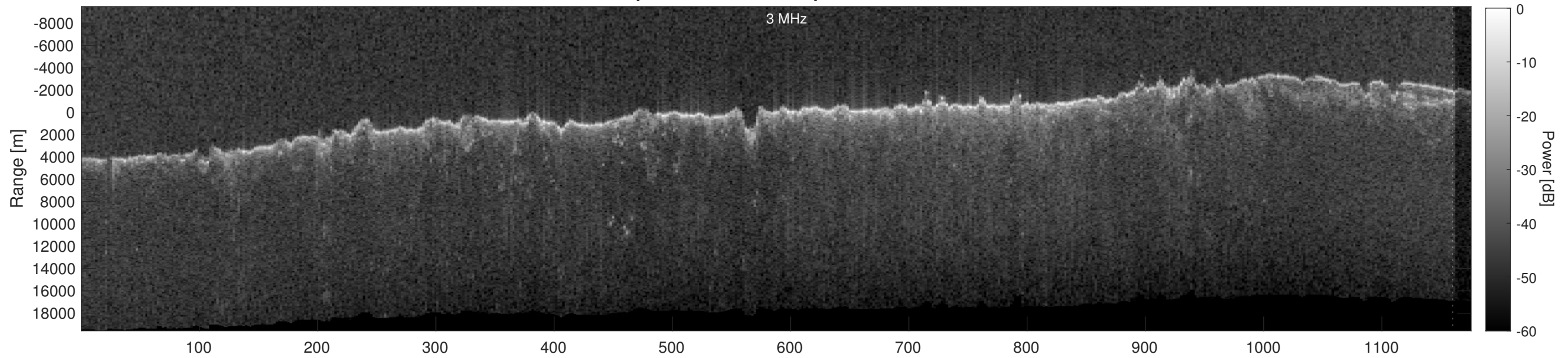
Orbit 2773, Depth-Corrected Cluttergram
