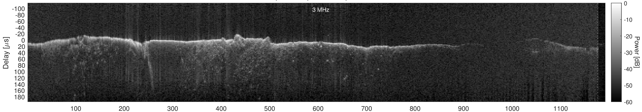
Orbit 2774, Window, Channel 2, Chapman
