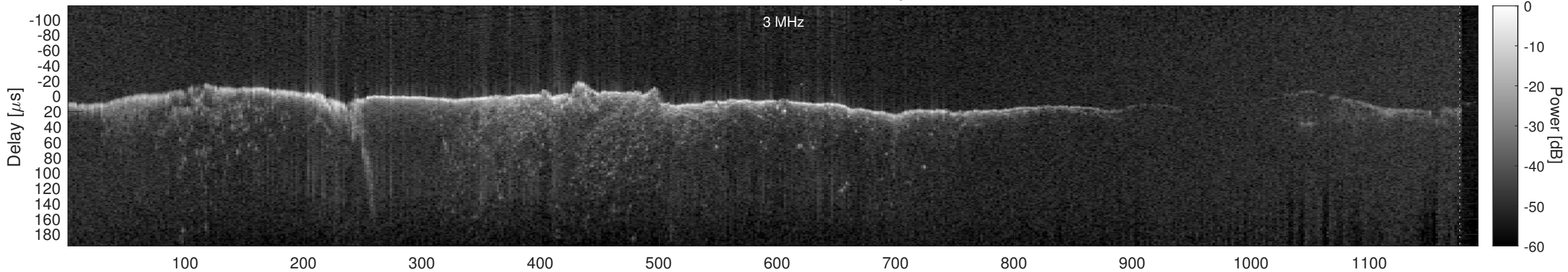
Orbit 2774, Window, Channel 2, Optimized
