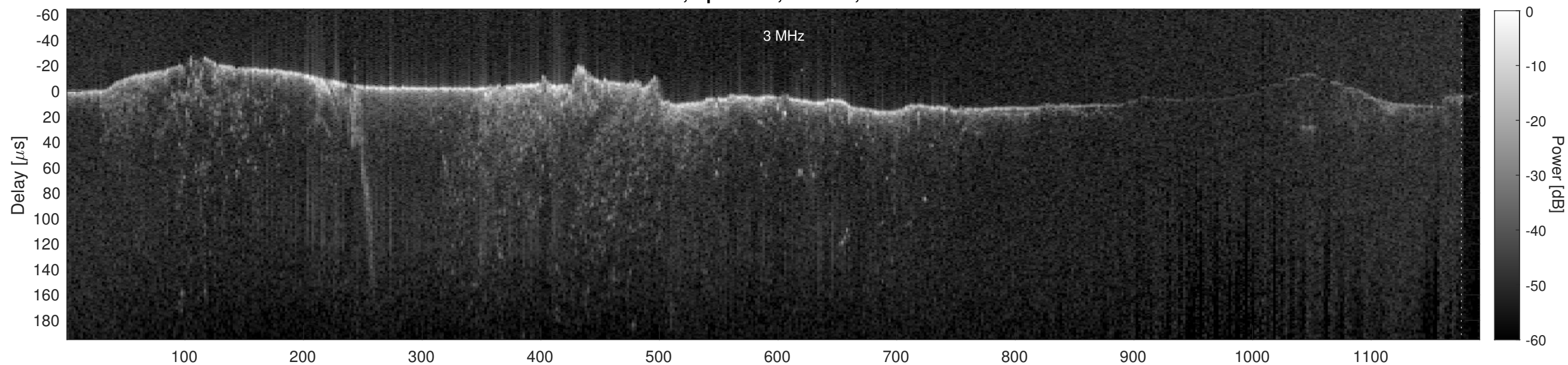
Orbit 2774, Cluttergram
