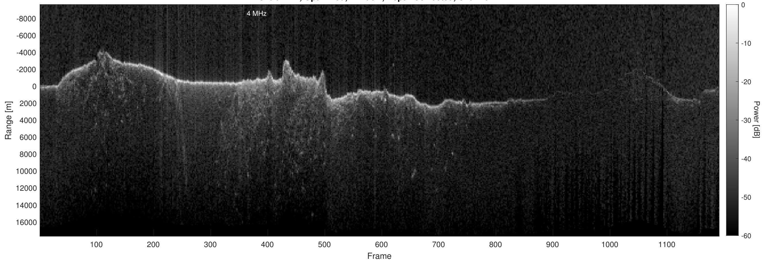
Orbit 2774, Optimized, Window, Depth-Corrected, Channel 2
