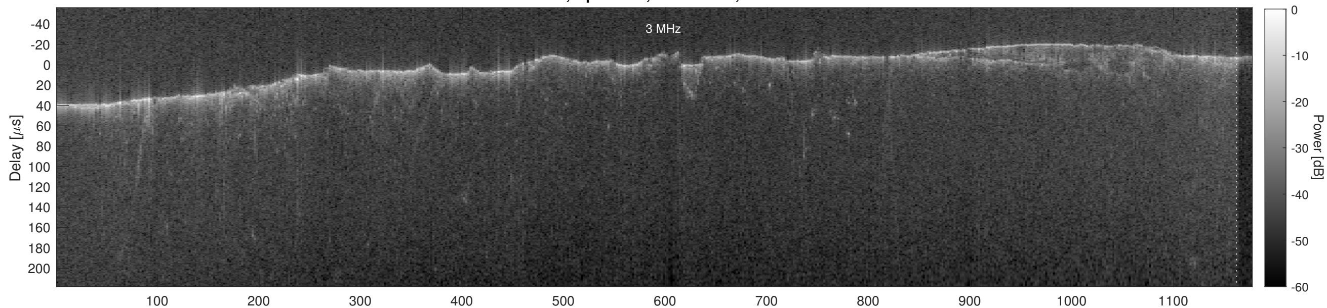
Orbit 2775, Cluttergram
