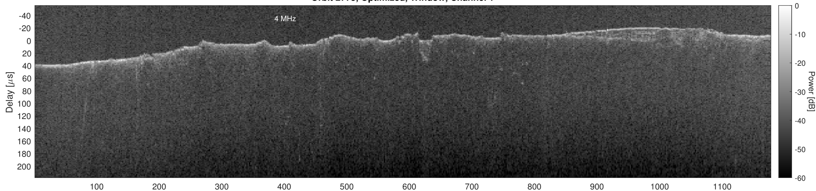
Orbit 2775, Optimized, Window, Channel 2
